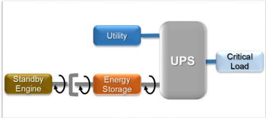
Figure 3a. Mechanically-coupled UPS with Standby Engine (DRUPS) Block Diagram.
