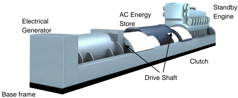
Figure 3b. Typical Mechanically-coupled DRUPS base frame layout
