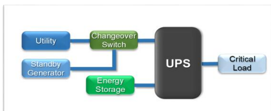
Figure 1. Generic UPS, Utility and Standby Generator arrangement.
