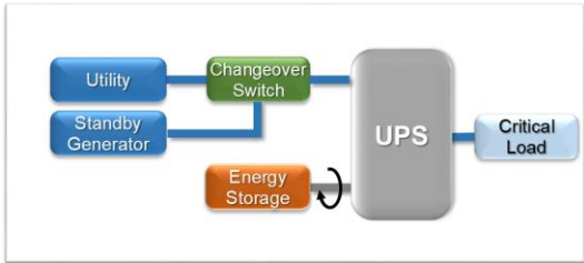
Figure 2. Mechanically-coupled UPS Block Diagram
