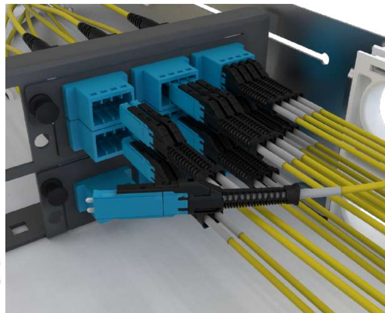
MDC SIDE (FRONT ENCLOSURE)
