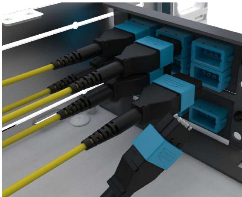
MDC SIDE (REAR ENCLOSURE)
