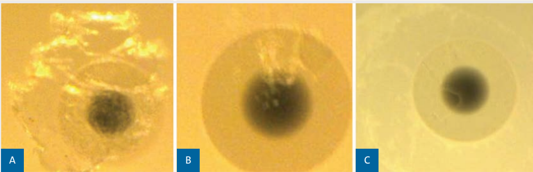
Figure 5: Particles deliberately placed over fibers in LC connectors to study effect of occlusion on IL: (a) Delrin®, (b) Ultem®, (c) skin flake.
